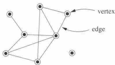
Fig. 1.1 A small example network with eight vertices and ten edges.
