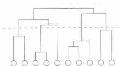
Fig. 3.5 An example of a dendrogram showing the hierarchical clustering of ten vertices. A horizontal cut through the dendrogram, such as that denoted by the dotted line, splits the vertices into a set of communities, five in this case.
