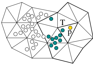
Figure 13: Collision detection between a particle (yellow) and a subset of the particles of the existing cluster (green).
