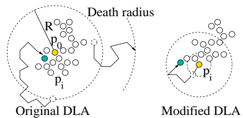
Figure 12: The original and modified DLA algorithms.
