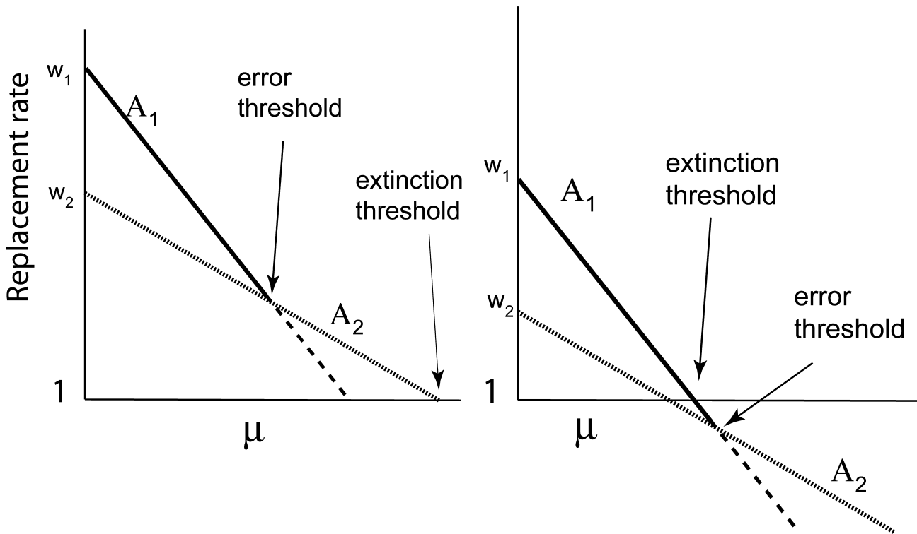
Figure 4. Extinction versus Error Catastrophe
