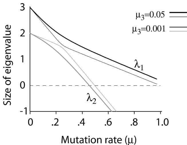
Figure 7. Eigenvalues When a Small Level of Back Mutation Occurs In contrast to the case of no back mutation in Figure 3, the eigenvalues here do not cross but change slope as they approach each other. The dark curves (upper) correspond to the maximum eigenvalue ( \lambda_1 ) and the light curves (lower) to the smaller eigenvalue. The thick, outer curves are drawn for a back mutation rate of \mu_3 = 0.05 , and the thin, inner curves for \mu_3 = 0.001 . The effect of increasing back mutation is clearly seen as increasing the minimum distance between the eigenvalue functions. Other parameters are the same as for the right side of Figure 3: w_1 = 3.0 , w_2 = 2 , and k = 2 .
