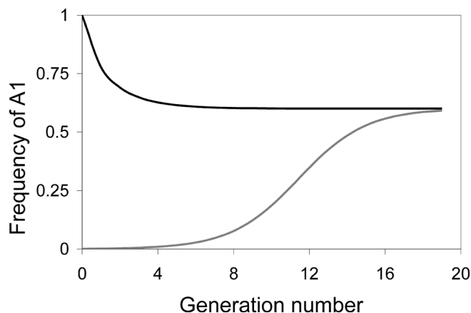
Figure 2. Dynamic Approach to the Quasispecies Equilibrium, for the Genotypes Illustrated in Figure 1
