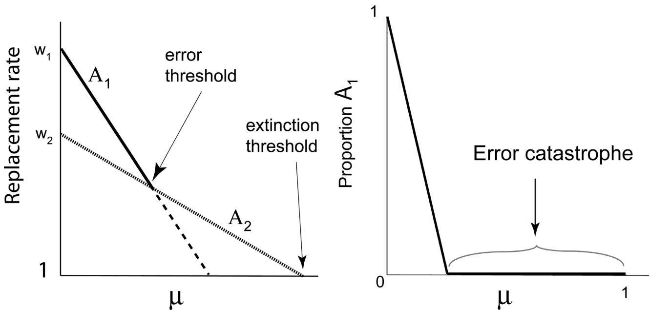
Figure 3. The Error Threshold and Error Catastrophe
